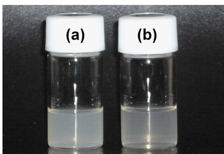
FIG. 8. (Color online) Photos of AZO NPs dispersed in chloroform at concentration of 10 mg/mL. (a) AZO NPs (10 input mol %) and (b) ZnO NPs.
