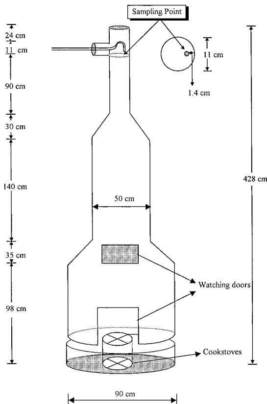
FIGURE 1. Hood and sampling port.
