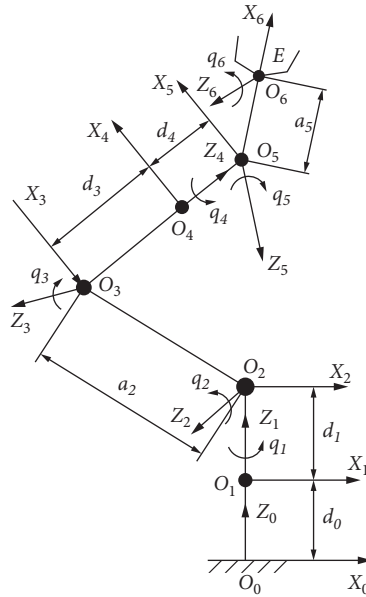
FIGURE 9: Kinematics model.
