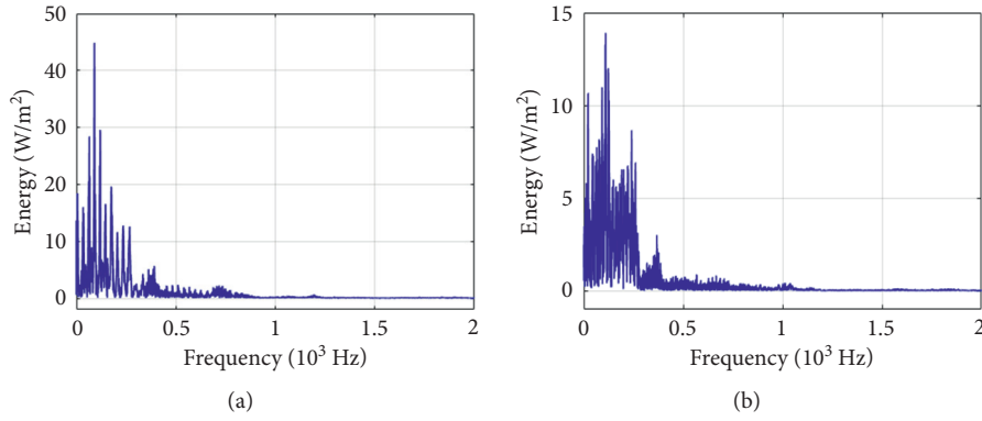
FIGURE 4: Sound energy of the word “Quay” and the word “Phải”.
