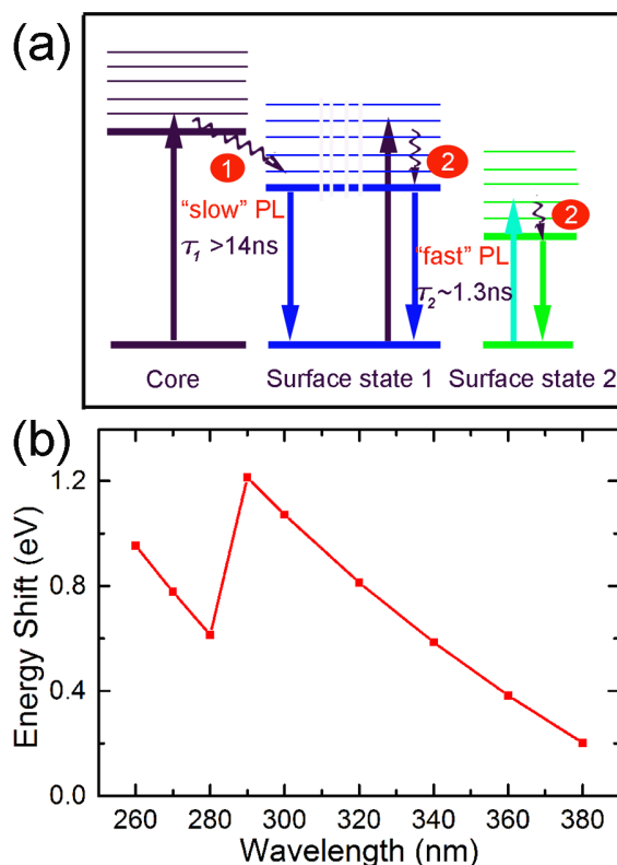
Fig. 4 - (a) Schematics of the carrier dynamics in C-dots. There are two different pathways of electron-hole radiative recombination with distinct relaxation time scales: (1) relaxation of carriers from carbogenic core onto the surface states with a slow decay ( \tau_1 > 14 ns), (2) direct radiative recombination of the carriers on surface states with a fast decay ( \tau_2 \sim 1.3 ns). (b) The dependence of the energy shift (difference of excitation energy and emission energy) versus excitation wavelength.
