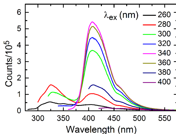
Fig. 2 - The steady-state PL spectra of the as-prepared C-dots in solution.
